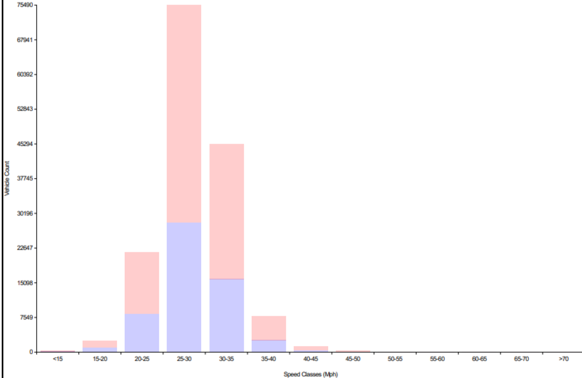
Vehicle Counts By Speed Class Traffic Overview from Wed Feb 1 2023 to Mon Jun 26 2023
