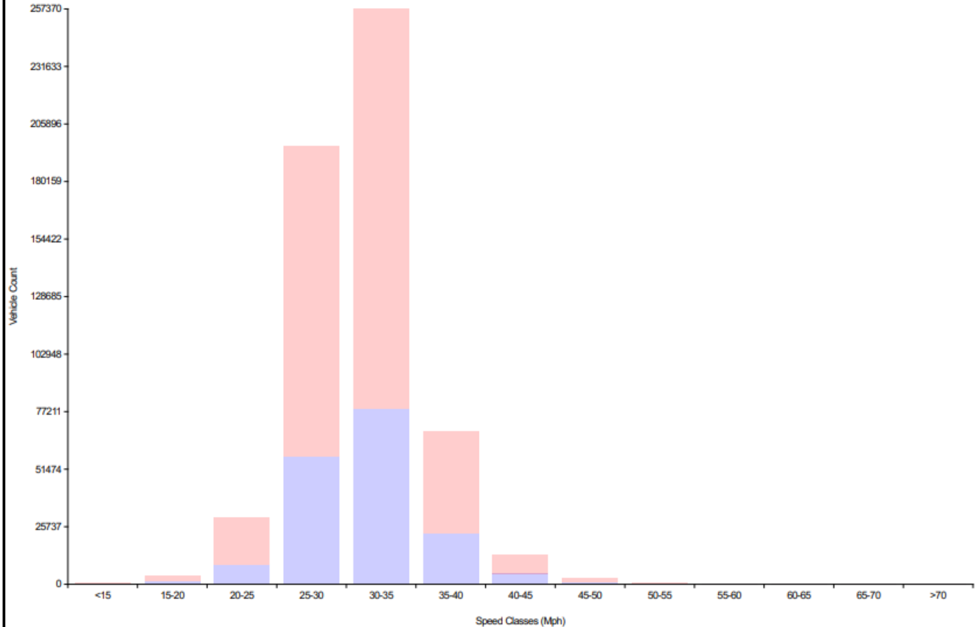
Vehicle Counts By Speed Class Traffic Overview from Wed Mar 21 2018 to Sat Jan 8 2022
